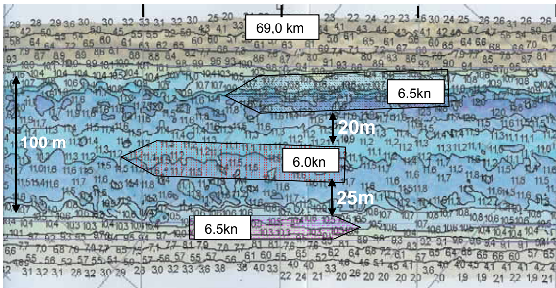
Figure 6. Second encounter of three vessels. RIROIL 5 is encountering ESTRADEN and WOLGASTER.
